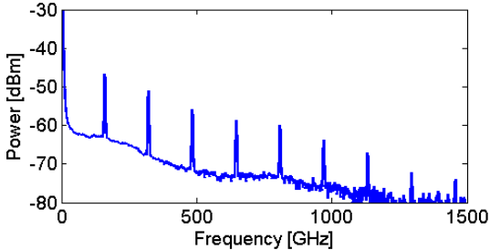
RF Spectrum
